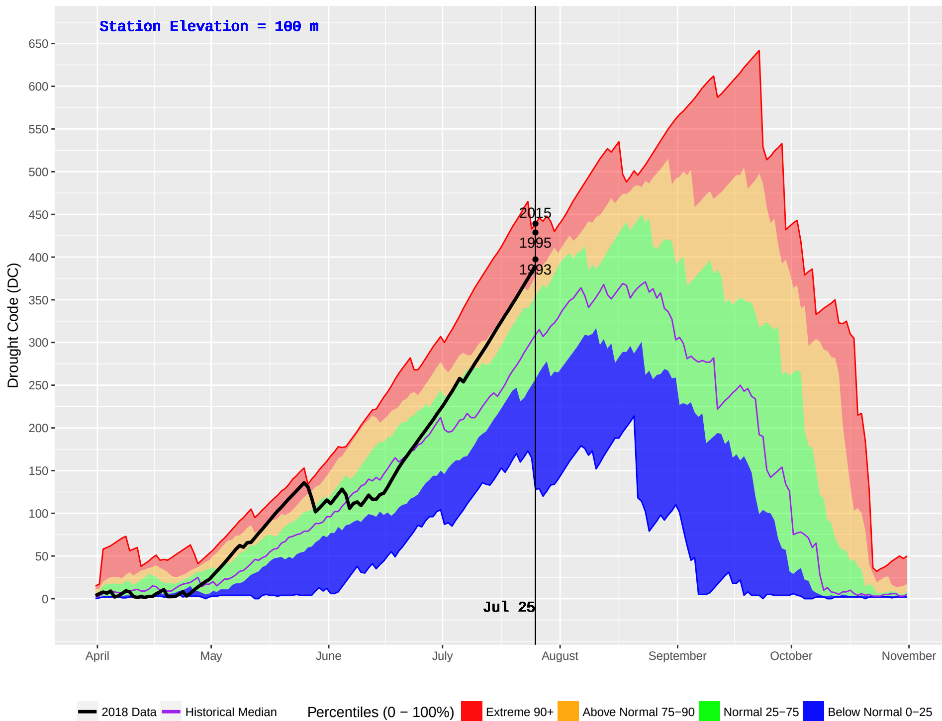
HONNA (93) : Historical (1986–2016) and Current (2018) Noon Drought Code (DC)
